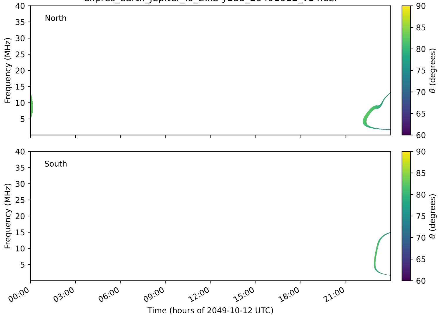
expres_earth_jupiter_io_txka-y235_20491012_v14.cdf
