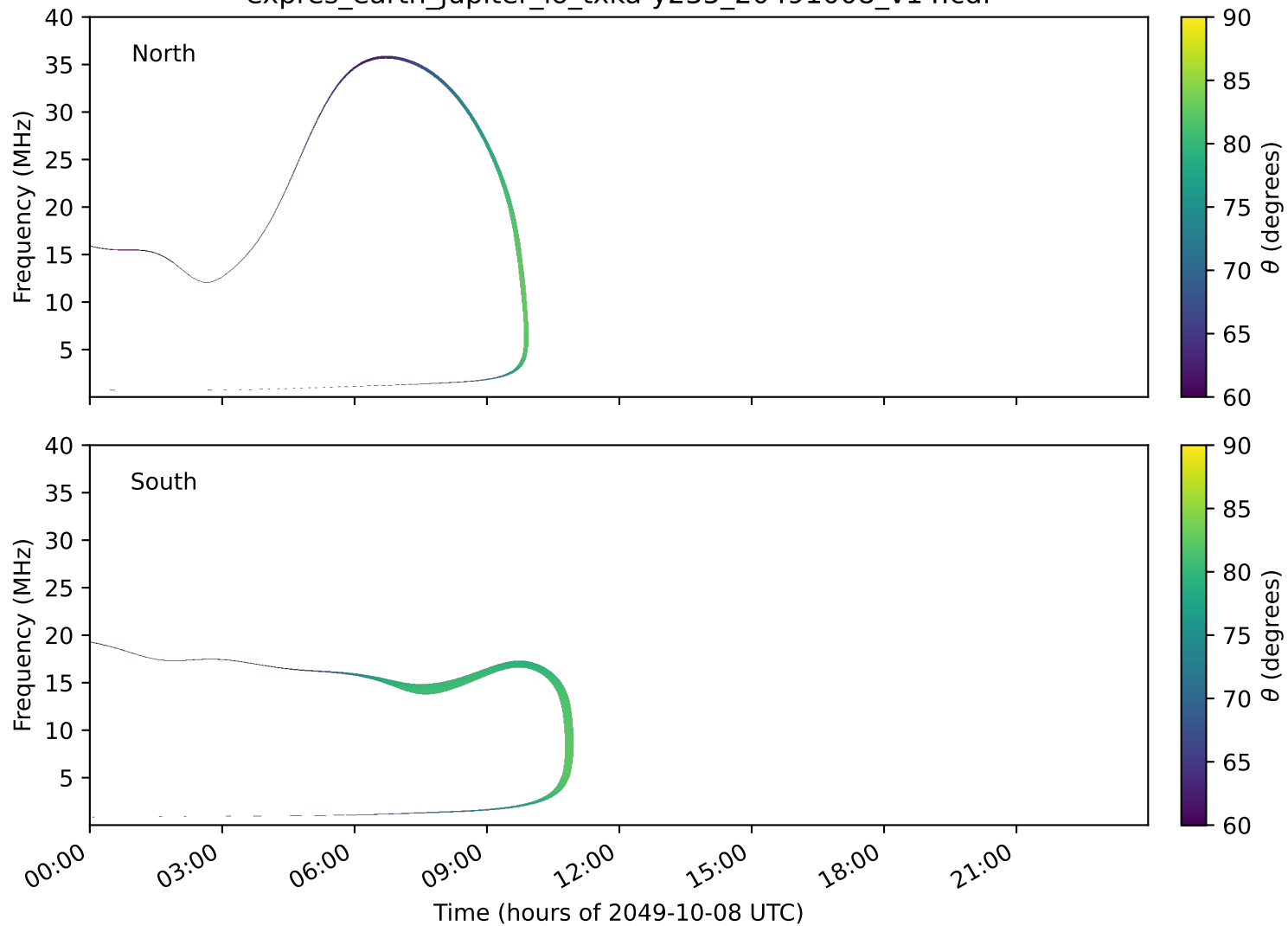
expres_earth_jupiter_io_txka-y235_20491008_v14.cdf
