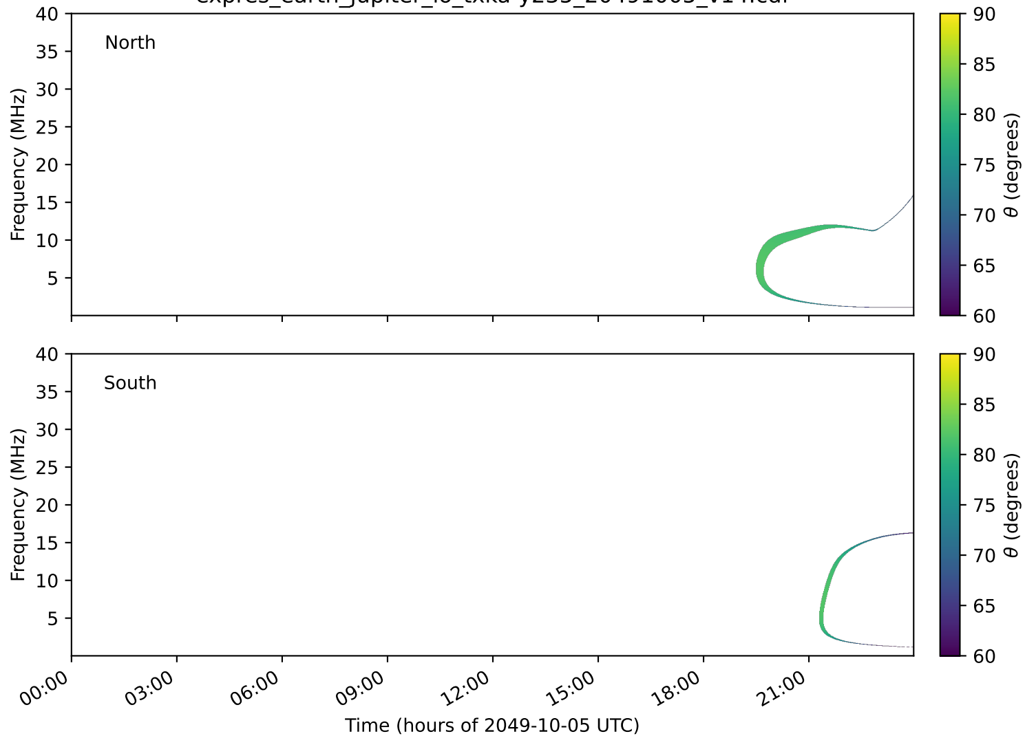
expres_earth_jupiter_io_txka-y235_20491005_v14.cdf
