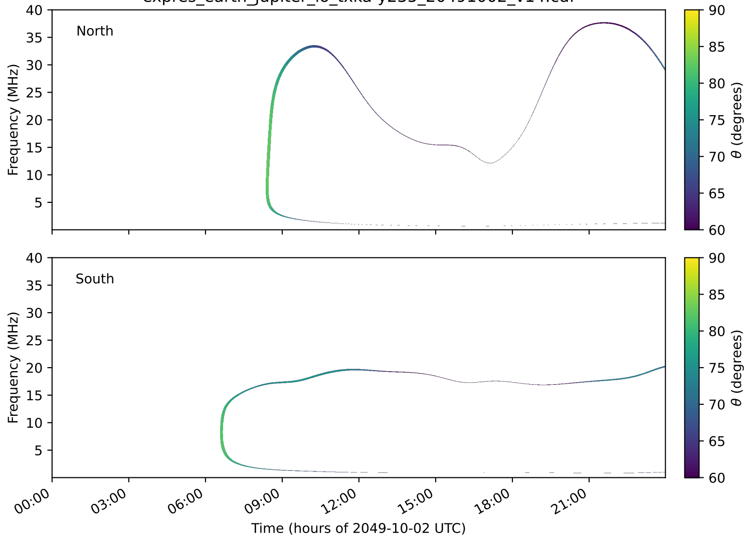
expres_earth_jupiter_io_txka-y235_20491002_v14.cdf
