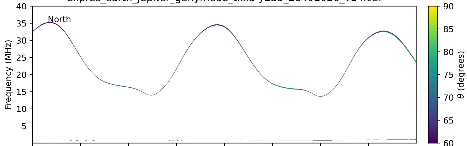
expres_earth_jupiter_ganymede_txka-y235_20491026_v14.cdf
