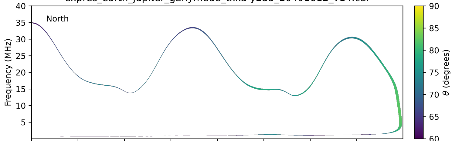
expres_earth_jupiter_ganymede_txka-y235_20491012_v14.cdf
