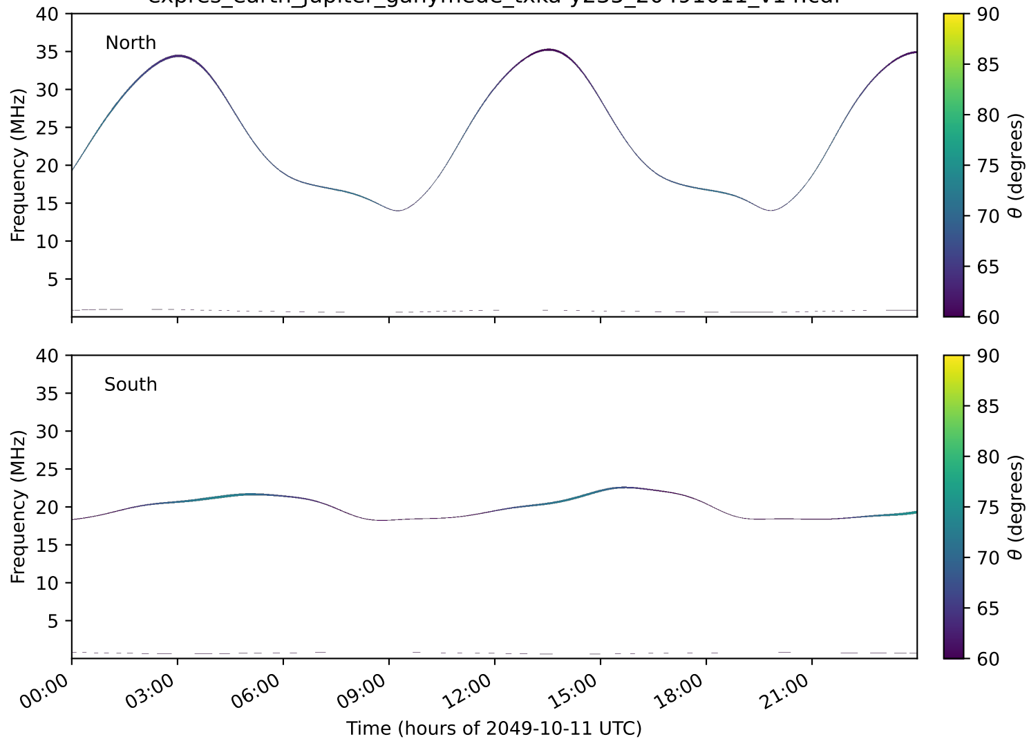
expres_earth_jupiter_ganymede_txka-y235_20491011_v14.cdf
