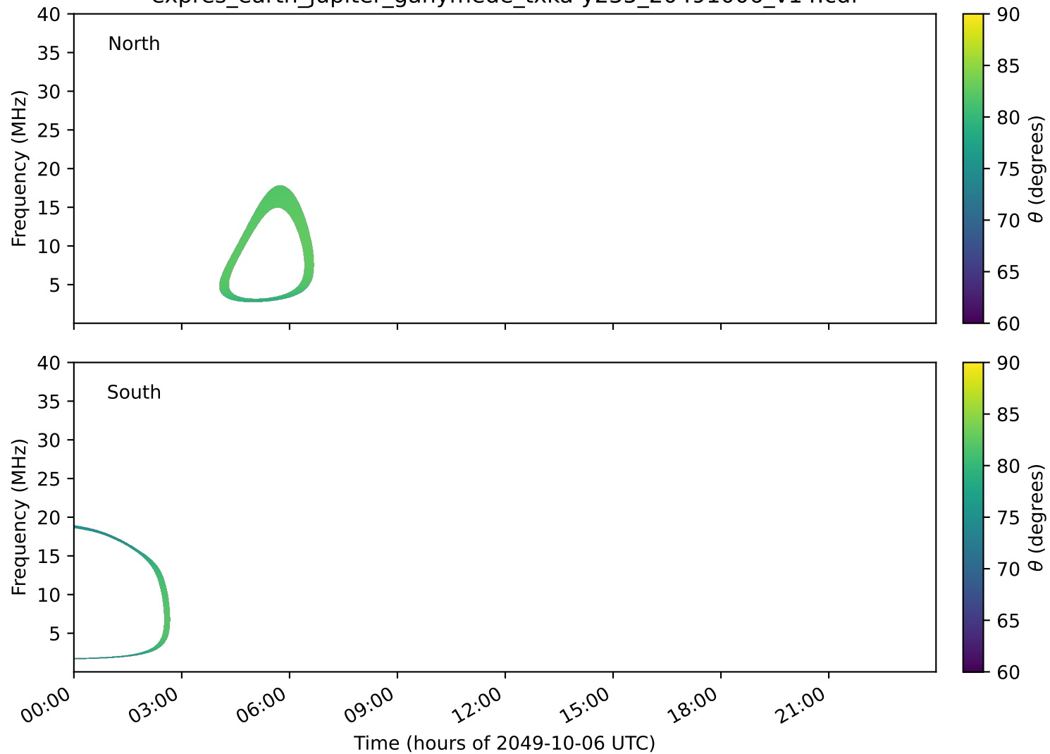
expres_earth_jupiter_ganymede_txka-y235_20491006_v14.cdf
