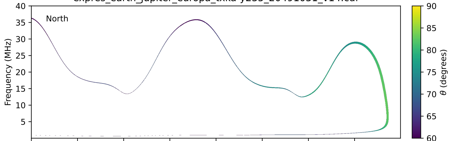
expres_earth_jupiter_europa_txka-y235_20491031_v14.cdf
