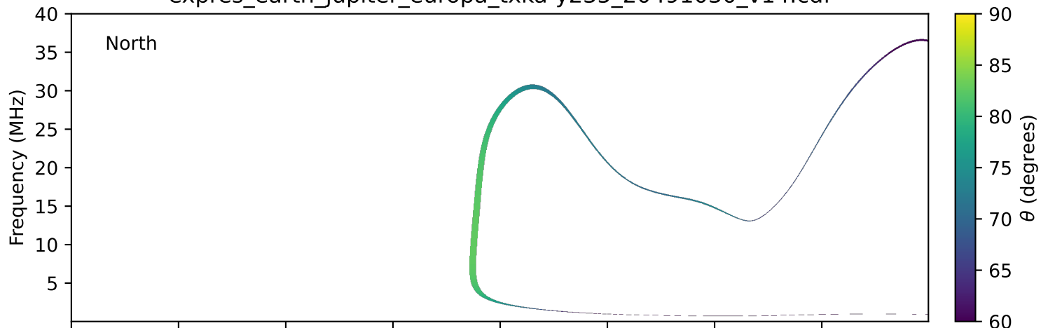
expres_earth_jupiter_europa_txka-y235_20491030_v14.cdf
