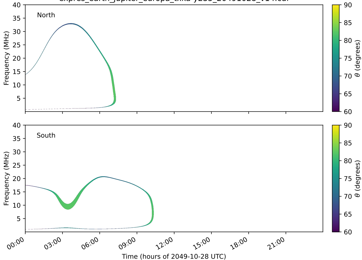
expres_earth_jupiter_europa_txka-y235_20491028_v14.cdf
