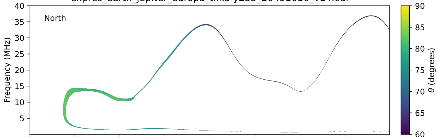
expres_earth_jupiter_europa_txka-y235_20491016_v14.cdf
