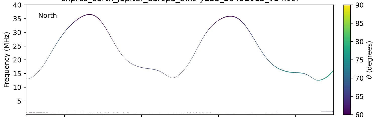
expres_earth_jupiter_europa_txka-y235_20491013_v14.cdf
