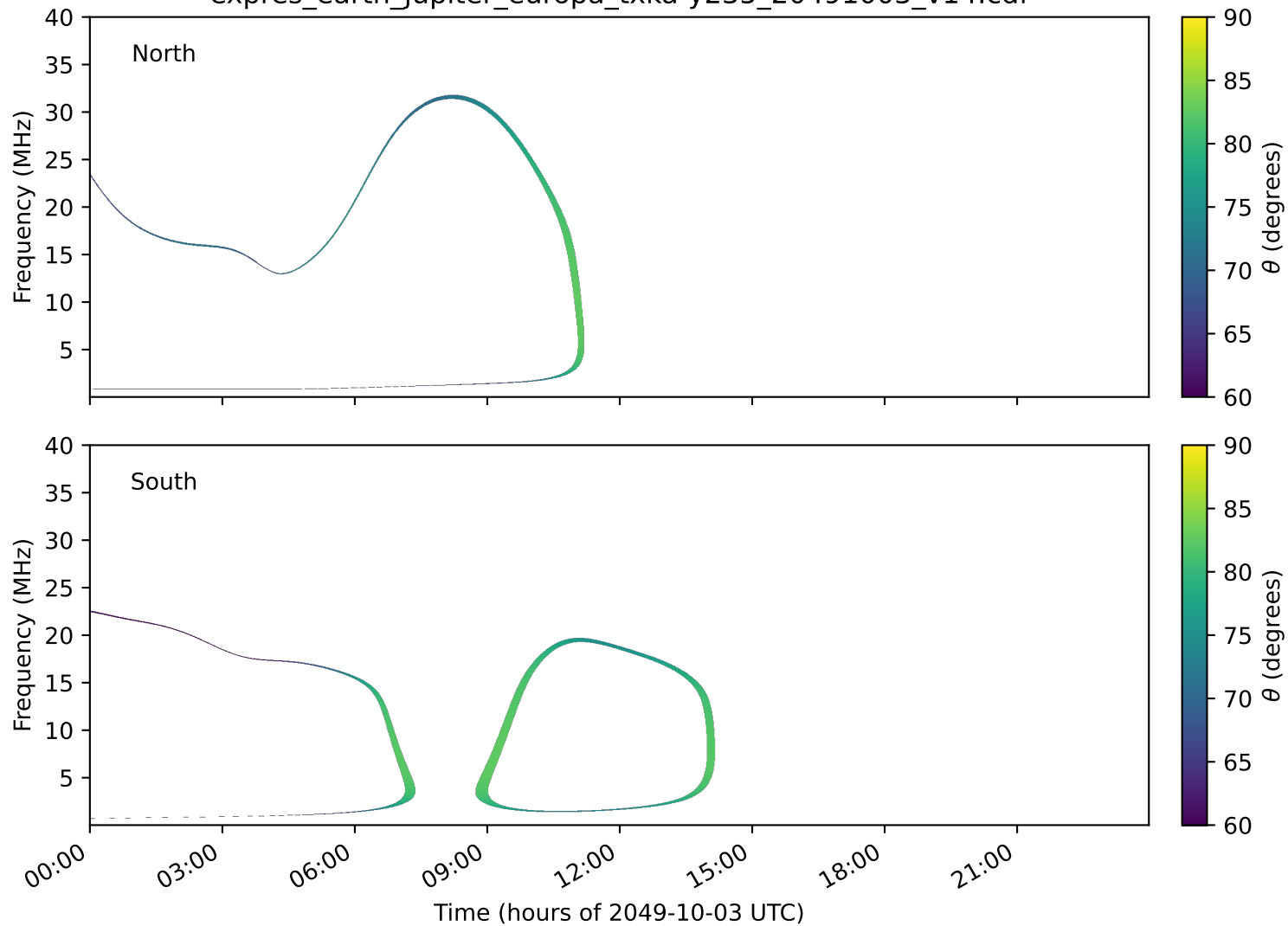
expres_earth_jupiter_europa_txka-y235_20491003_v14.cdf
