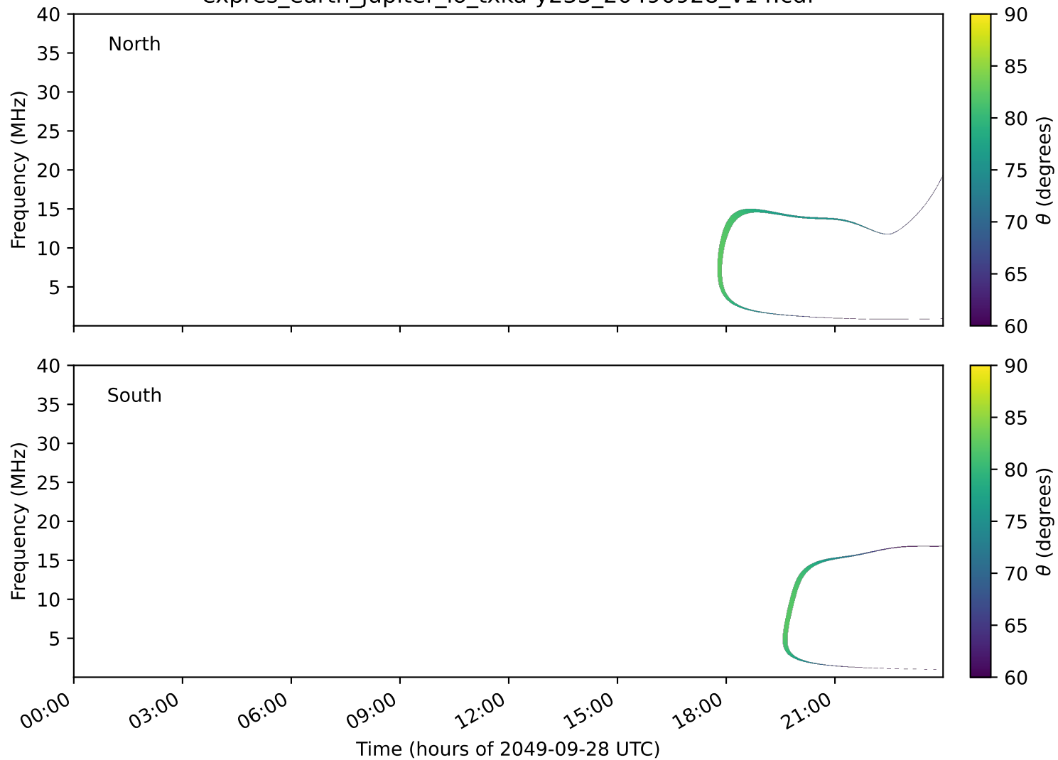
expres_earth_jupiter_io_txka-y235_20490928_v14.cdf
