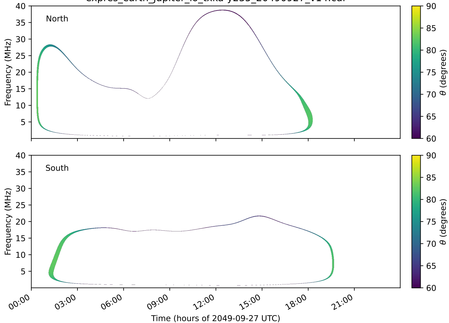
expres_earth_jupiter_io_txka-y235_20490927_v14.cdf
