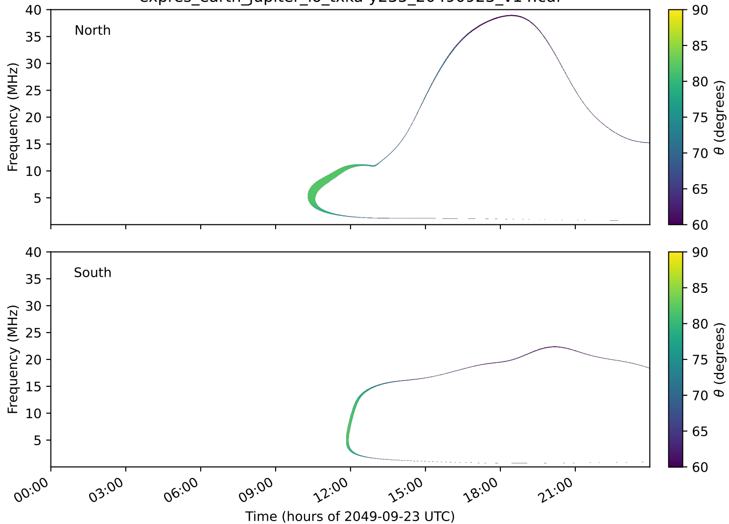
expres_earth_jupiter_io_txka-y235_20490923_v14.cdf
