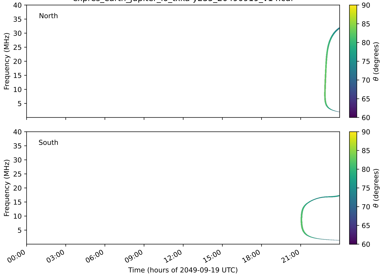
expres_earth_jupiter_io_txka-y235_20490919_v14.cdf
