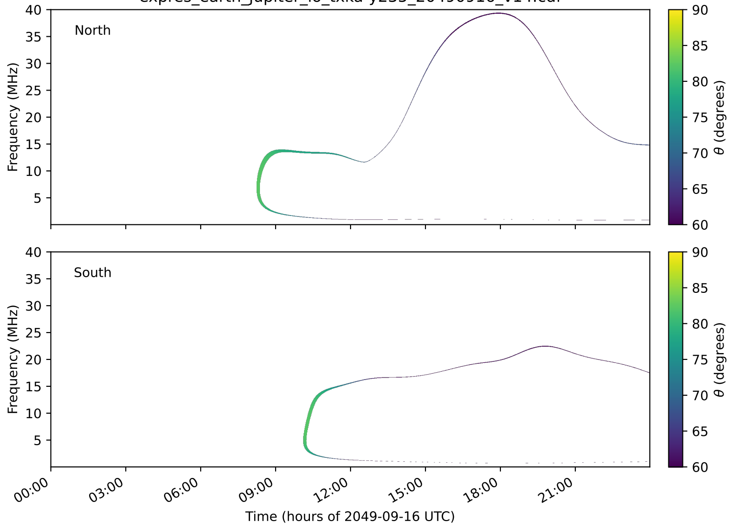
expres_earth_jupiter_io_txka-y235_20490916_v14.cdf
