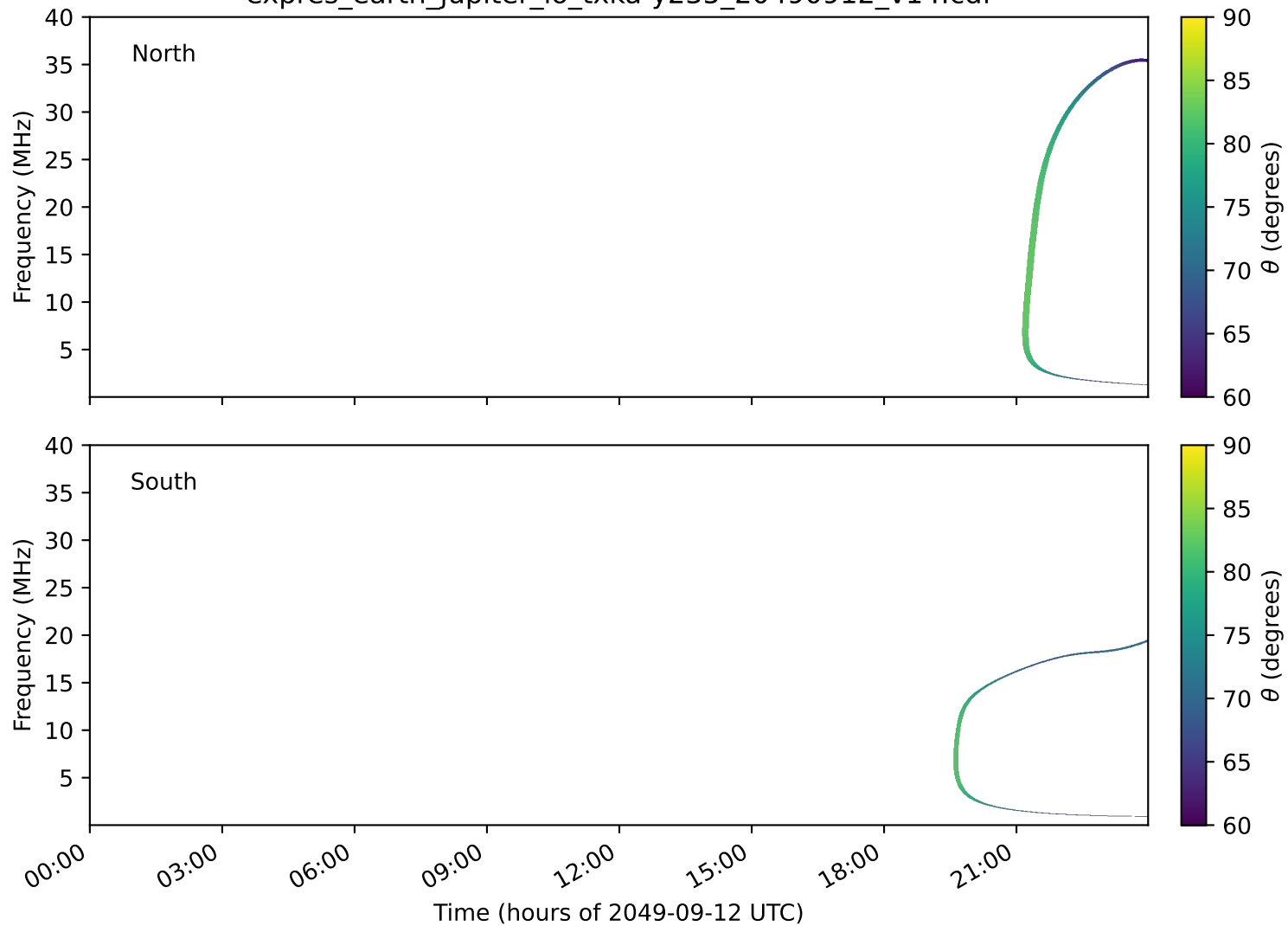
expres_earth_jupiter_io_txka-y235_20490912_v14.cdf
