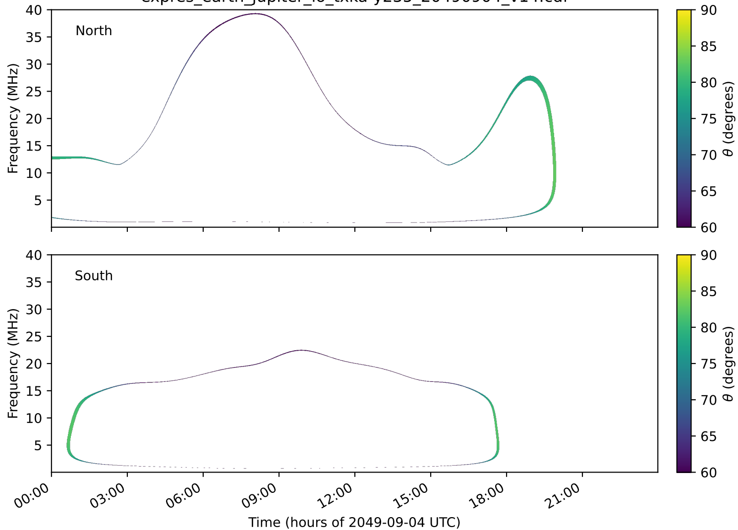
expres_earth_jupiter_io_txka-y235_20490904_v14.cdf
