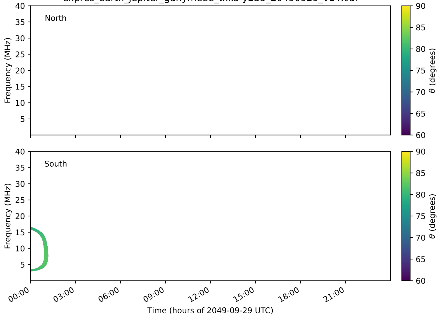
expres_earth_jupiter_ganymede_txka-y235_20490929_v14.cdf
