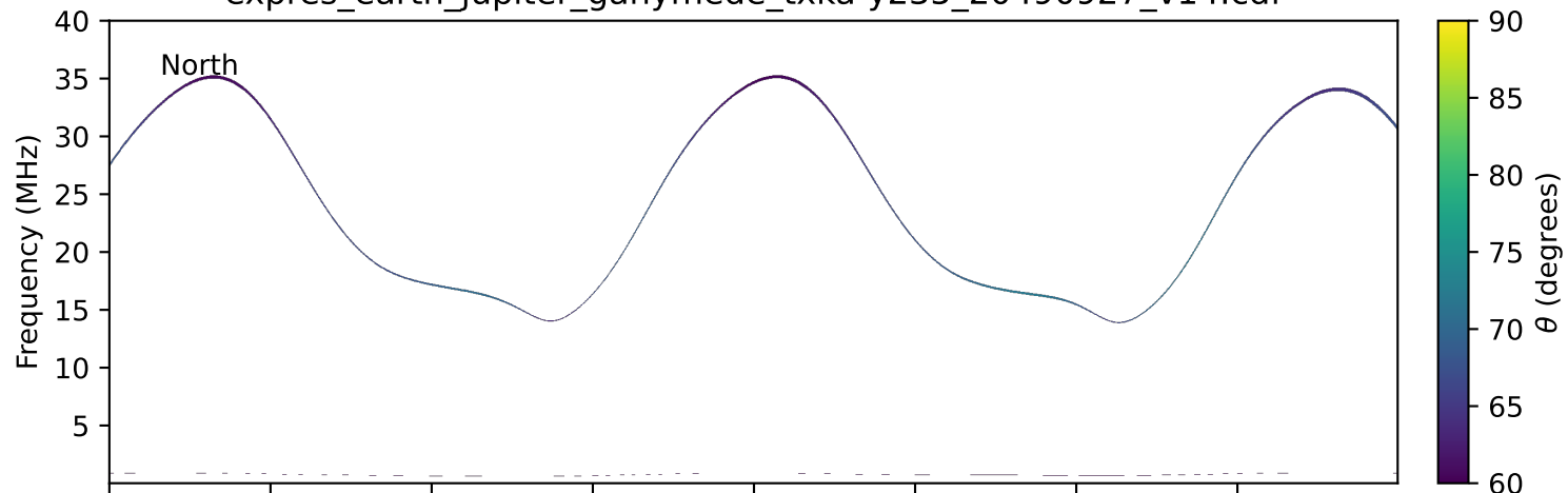
expres_earth_jupiter_ganymede_txka-y235_20490927_v14.cdf
