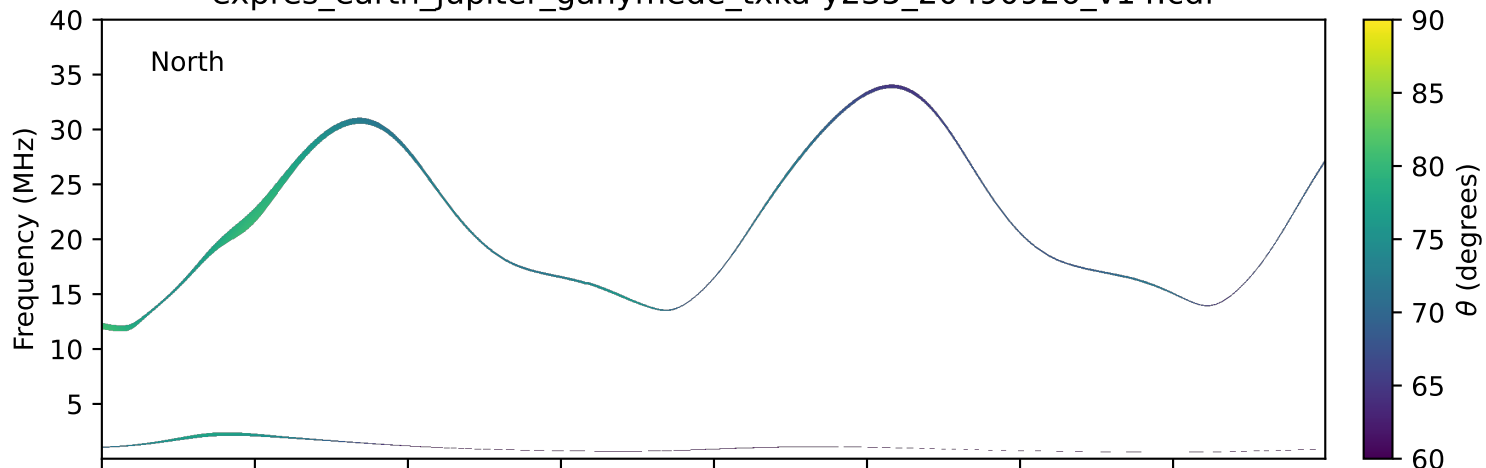
expres_earth_jupiter_ganymede_txka-y235_20490926_v14.cdf
