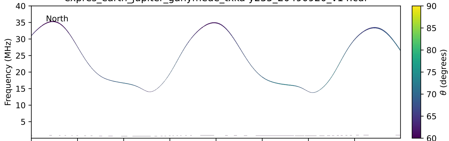
expres_earth_jupiter_ganymede_txka-y235_20490920_v14.cdf
