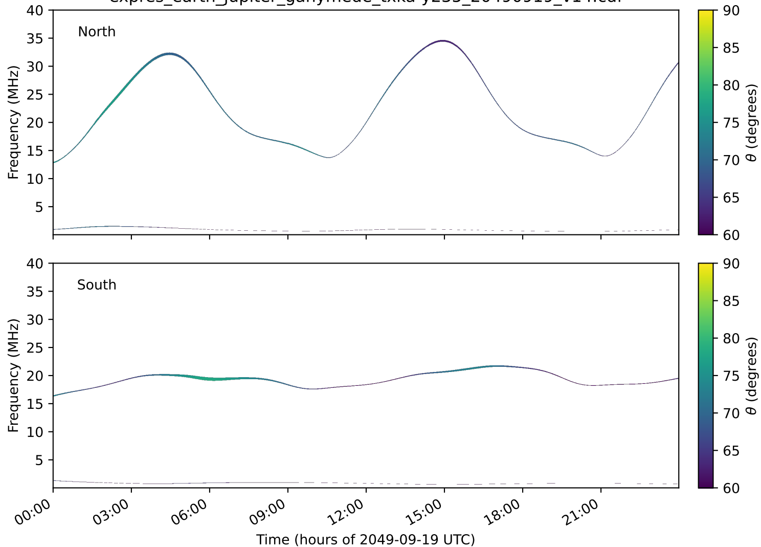
expres_earth_jupiter_ganymede_txka-y235_20490919_v14.cdf
