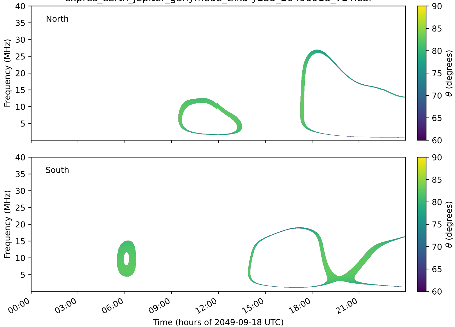
expres_earth_jupiter_ganymede_txka-y235_20490918_v14.cdf
