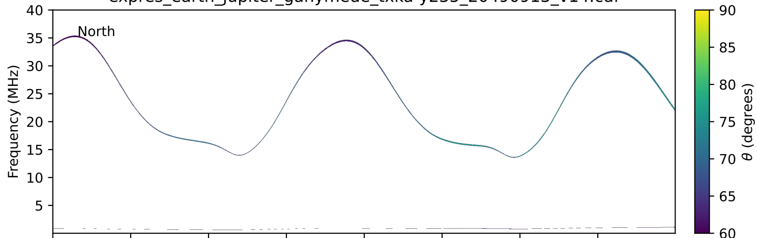
expres_earth_jupiter_ganymede_txka-y235_20490913_v14.cdf
