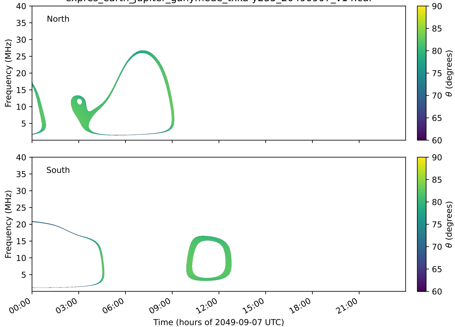
expres_earth_jupiter_ganymede_txka-y235_20490907_v14.cdf
