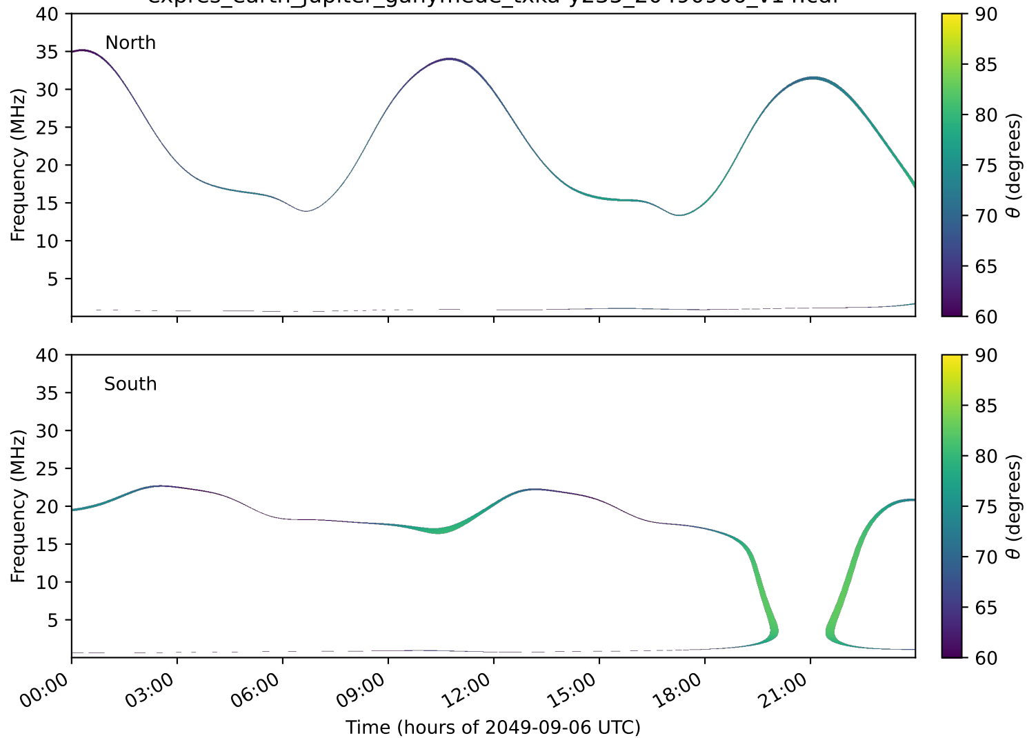
expres_earth_jupiter_ganymede_txka-y235_20490906_v14.cdf
