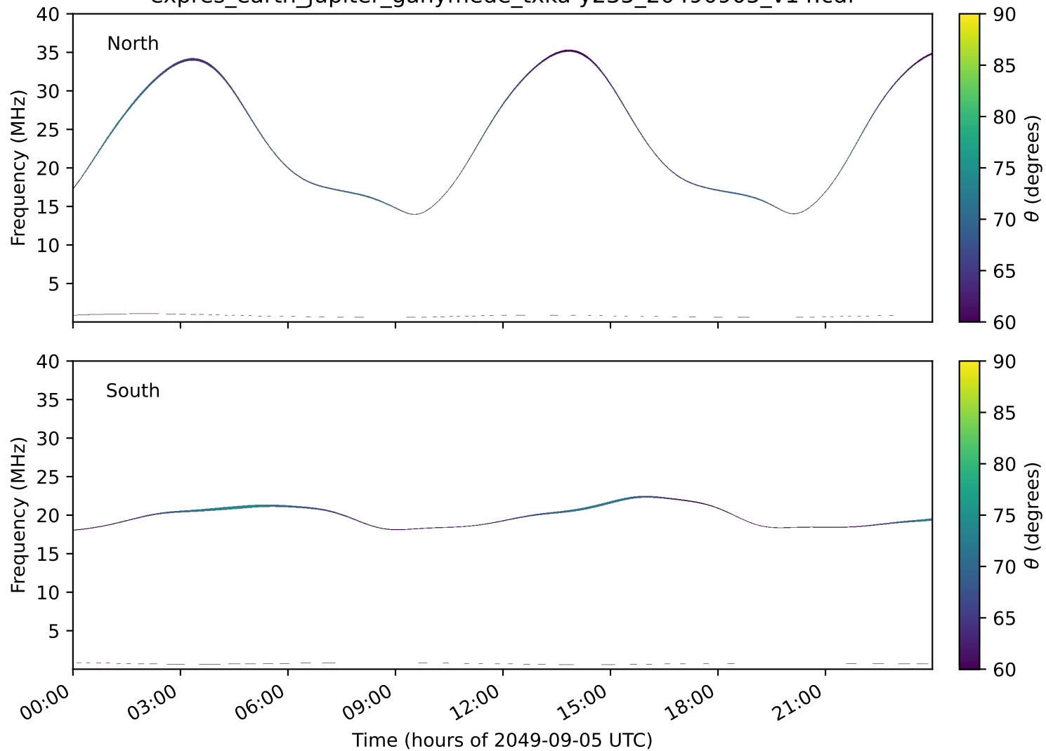
expres_earth_jupiter_ganymede_txka-y235_20490905_v14.cdf
