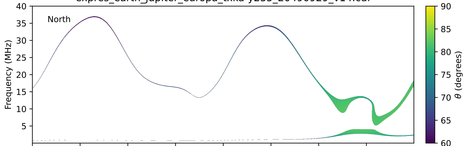
expres_earth_jupiter_europa_txka-y235_20490929_v14.cdf
