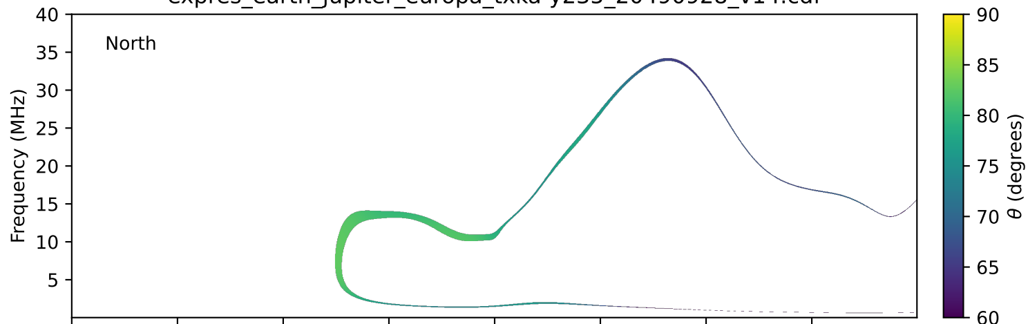
expres_earth_jupiter_europa_txka-y235_20490928_v14.cdf
