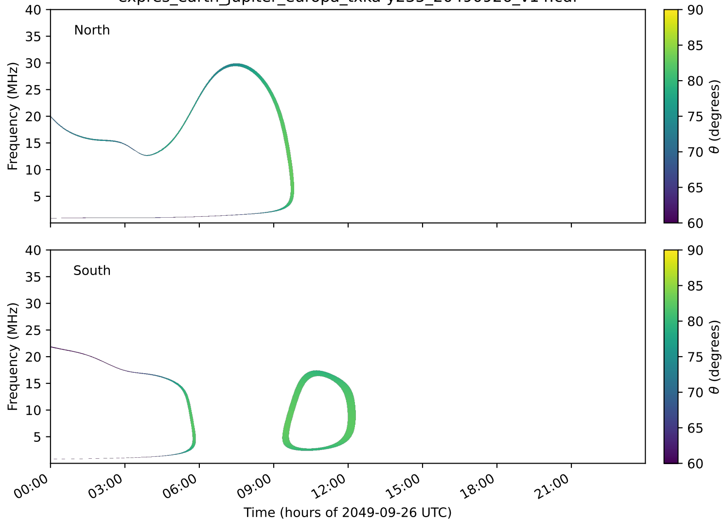
expres_earth_jupiter_europa_txka-y235_20490926_v14.cdf
