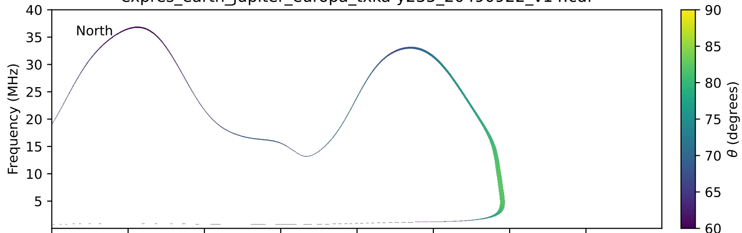
expres_earth_jupiter_europa_txka-y235_20490922_v14.cdf
