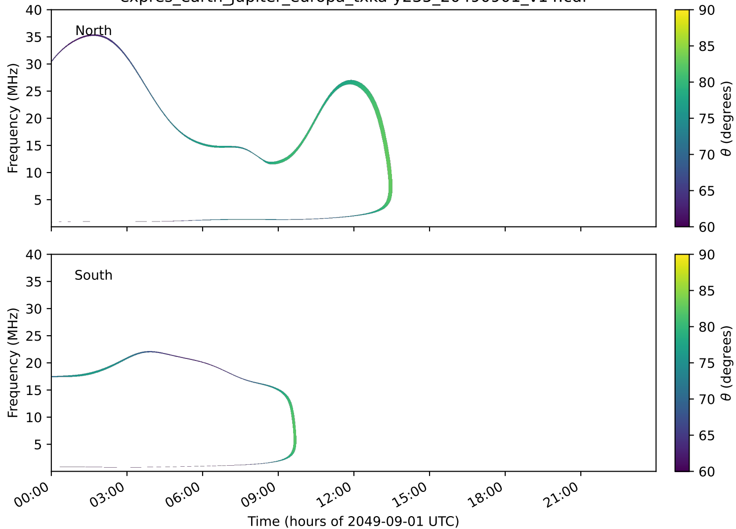
expres_earth_jupiter_europa_txka-y235_20490901_v14.cdf
