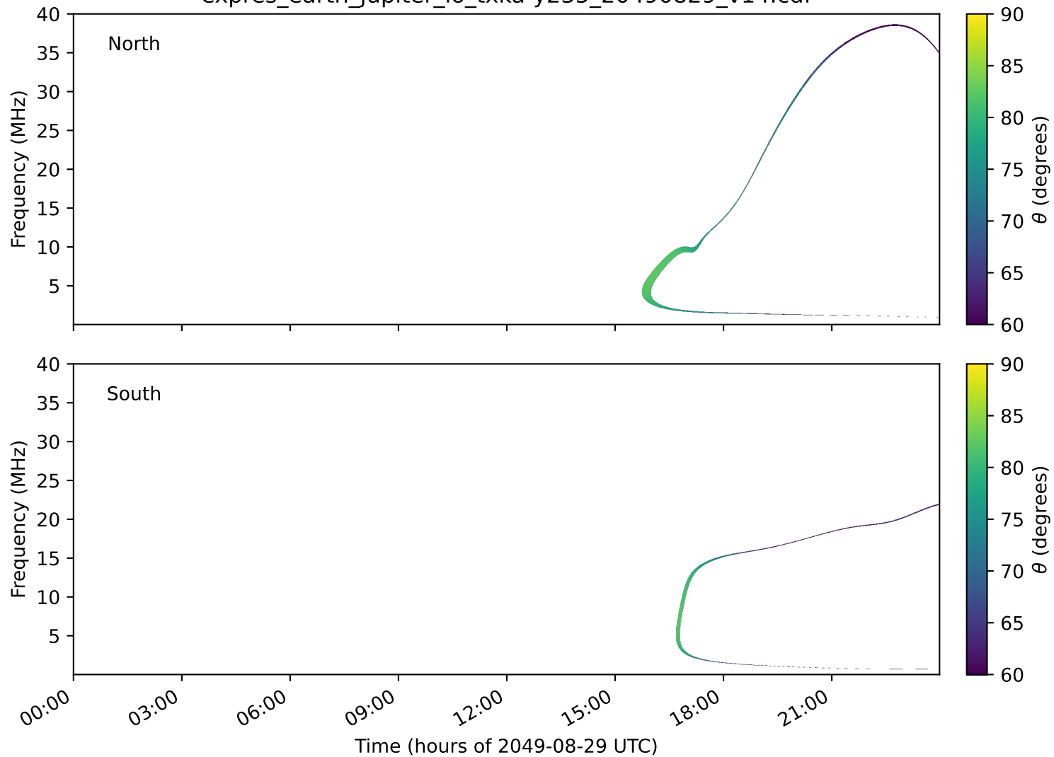
expres_earth_jupiter_io_txka-y235_20490829_v14.cdf
