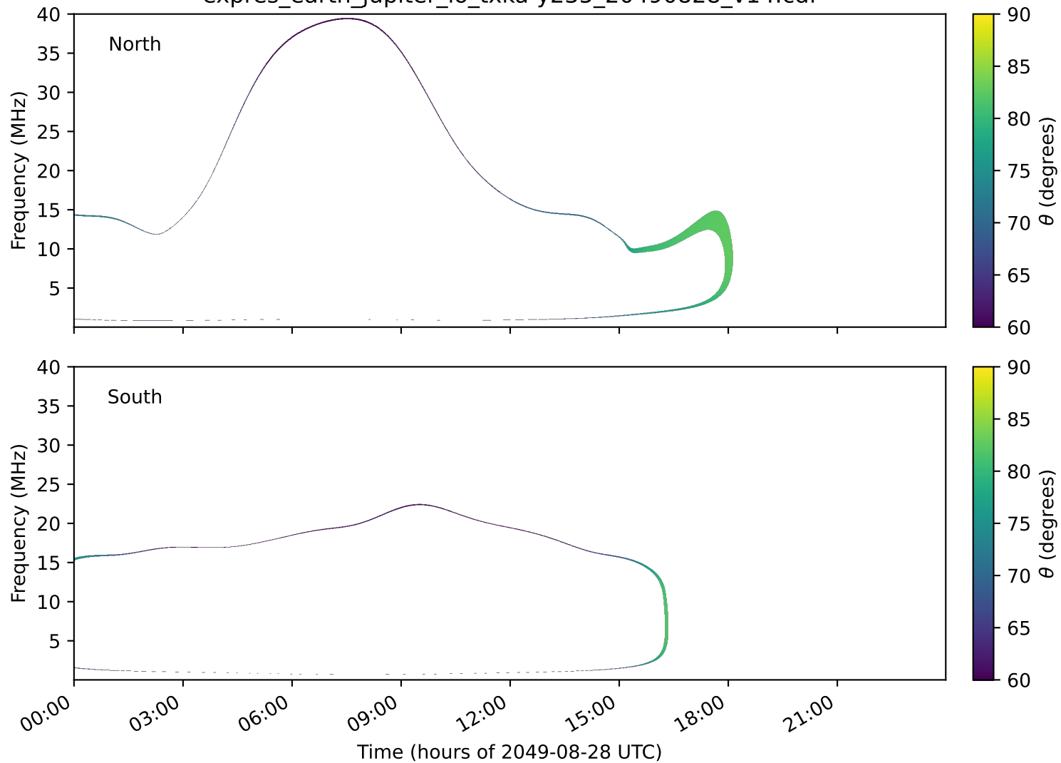
expres_earth_jupiter_io_txka-y235_20490828_v14.cdf
