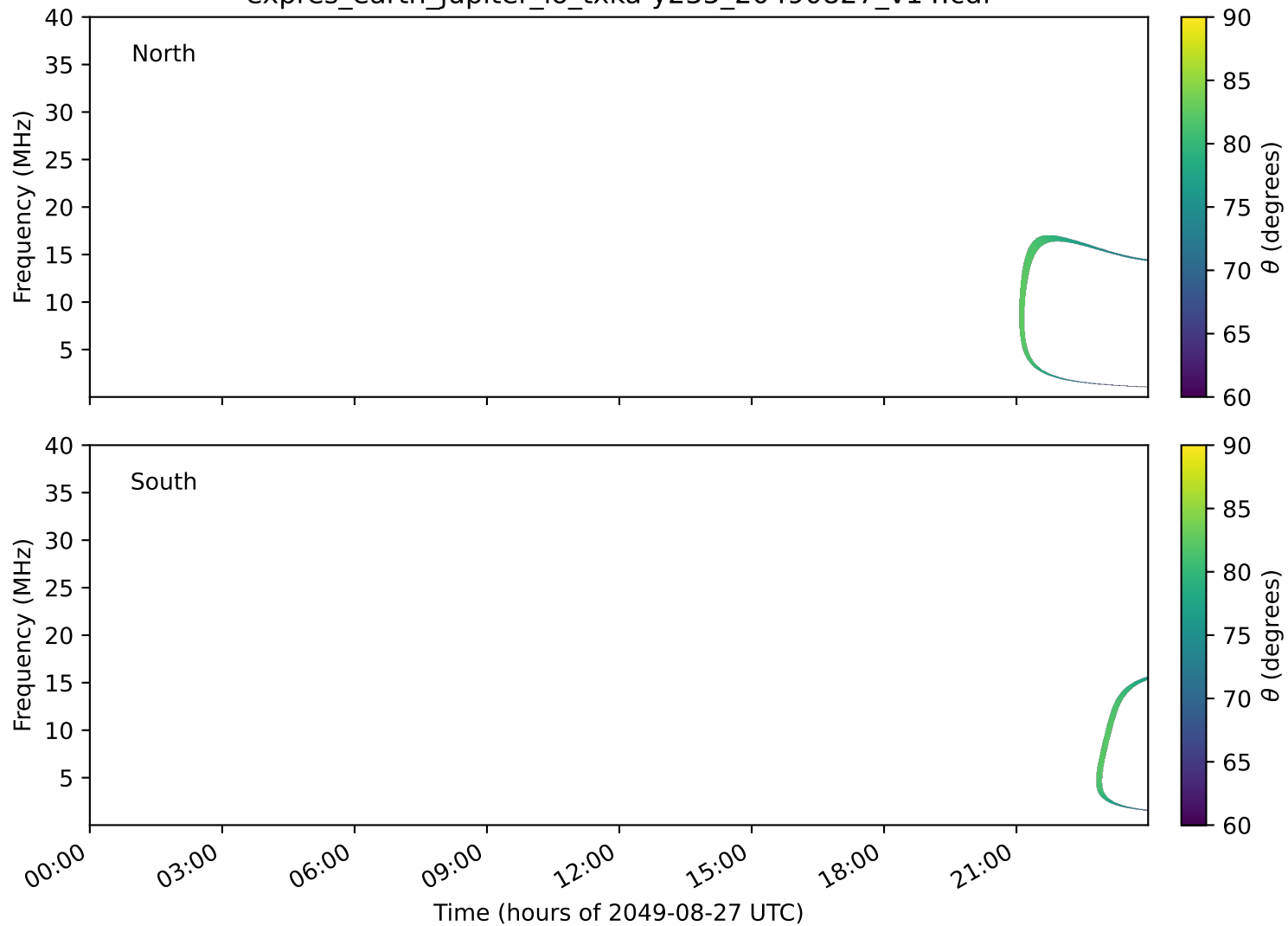
expres_earth_jupiter_io_txka-y235_20490827_v14.cdf
