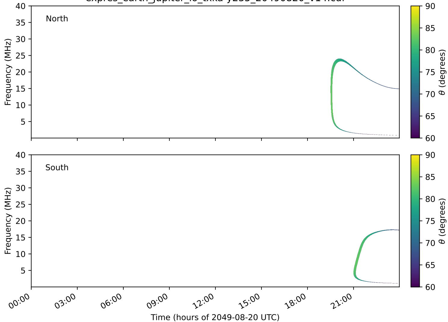
expres_earth_jupiter_io_txka-y235_20490820_v14.cdf
