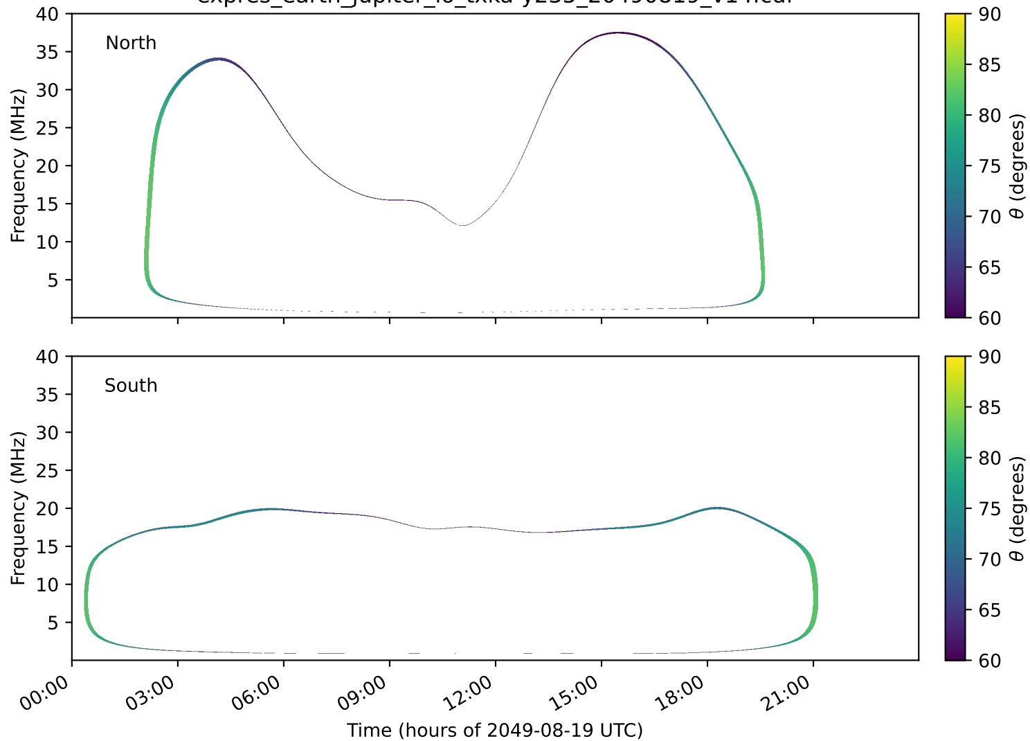
expres_earth_jupiter_io_txka-y235_20490819_v14.cdf
