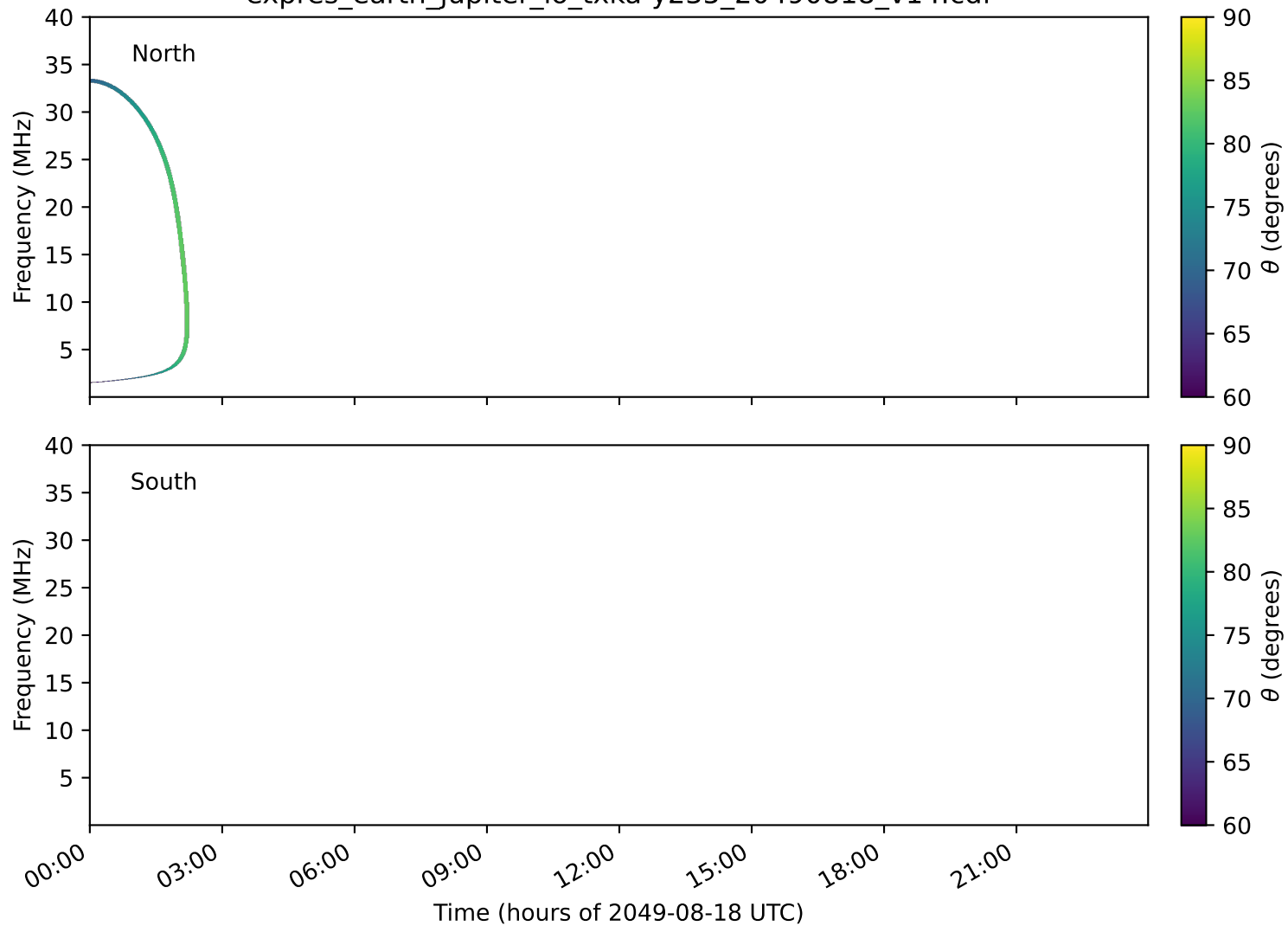
expres_earth_jupiter_io_txka-y235_20490818_v14.cdf
