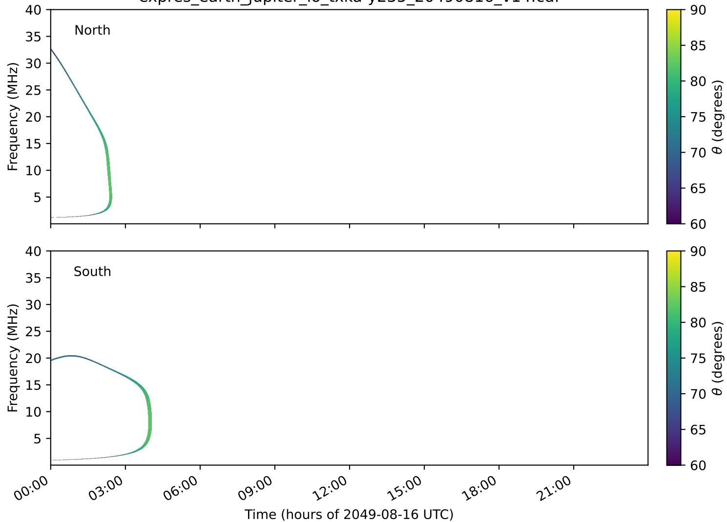
expres_earth_jupiter_io_txka-y235_20490816_v14.cdf
