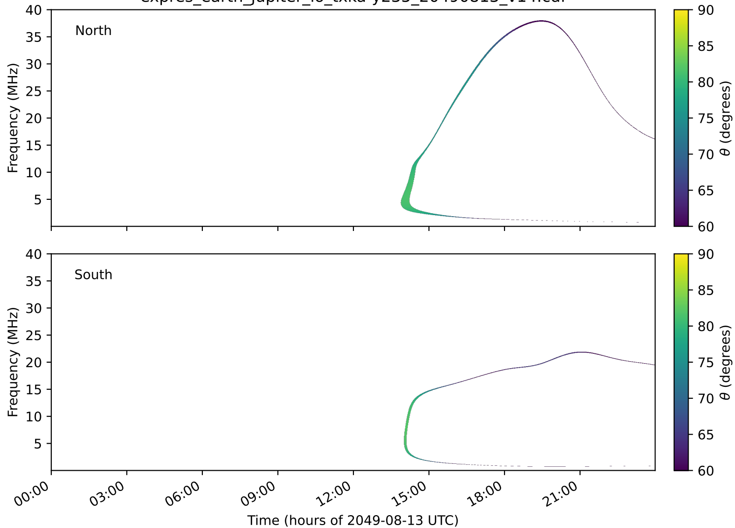
expres_earth_jupiter_io_txka-y235_20490813_v14.cdf
