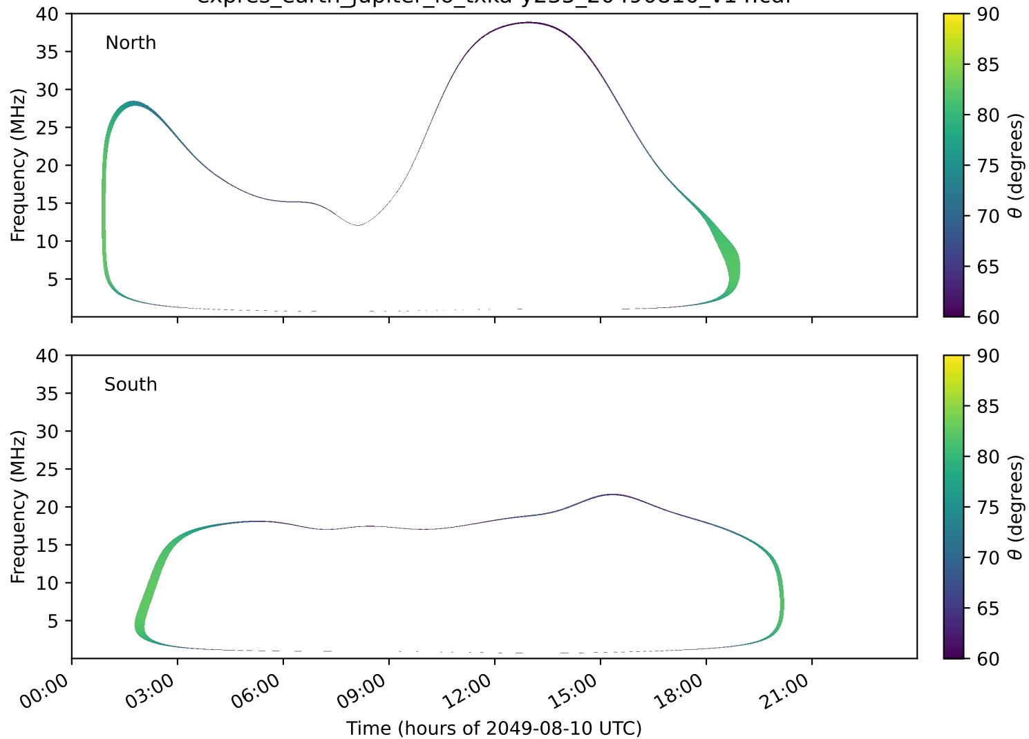
expres_earth_jupiter_io_txka-y235_20490810_v14.cdf
