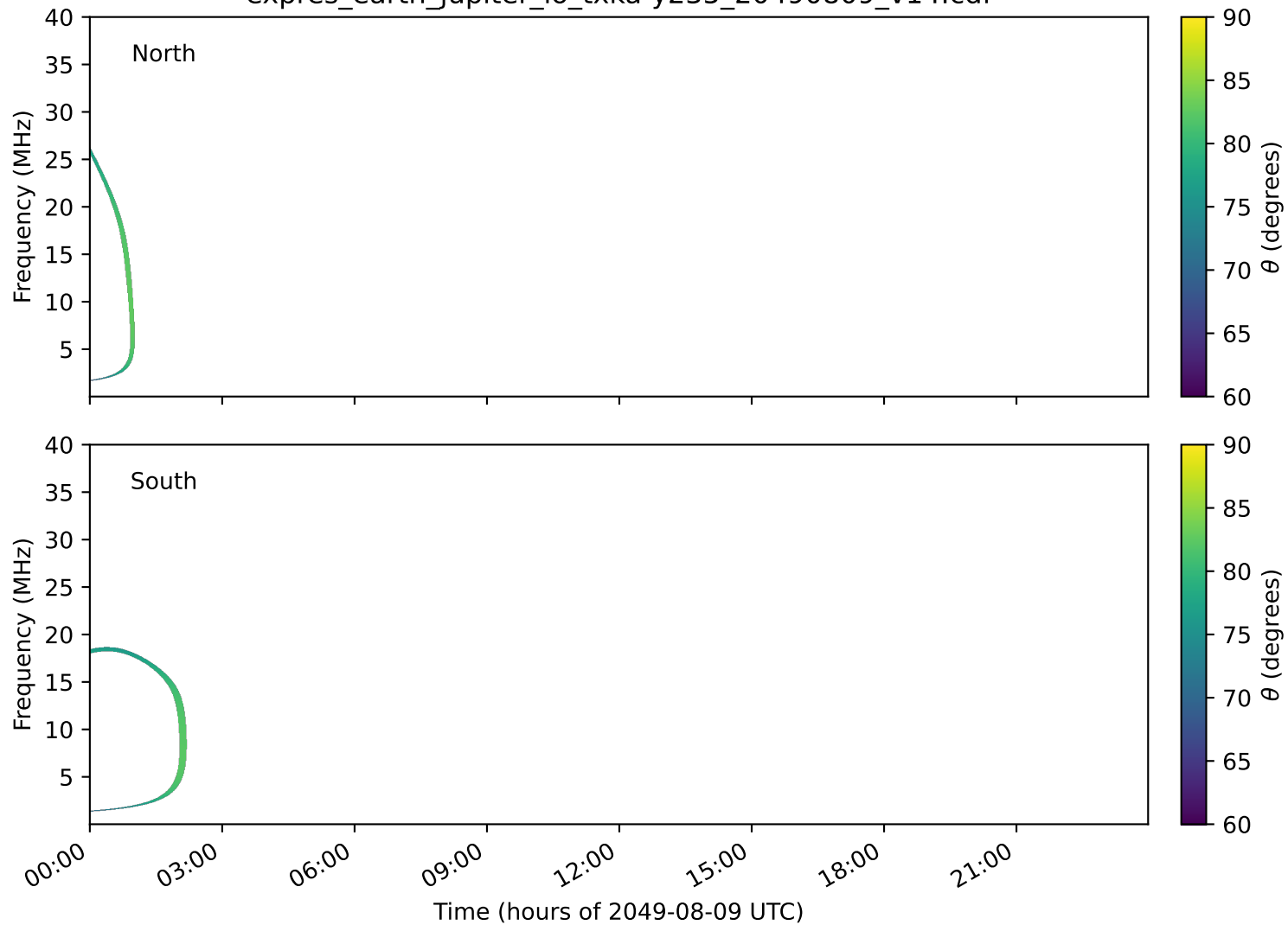
expres_earth_jupiter_io_txka-y235_20490809_v14.cdf
