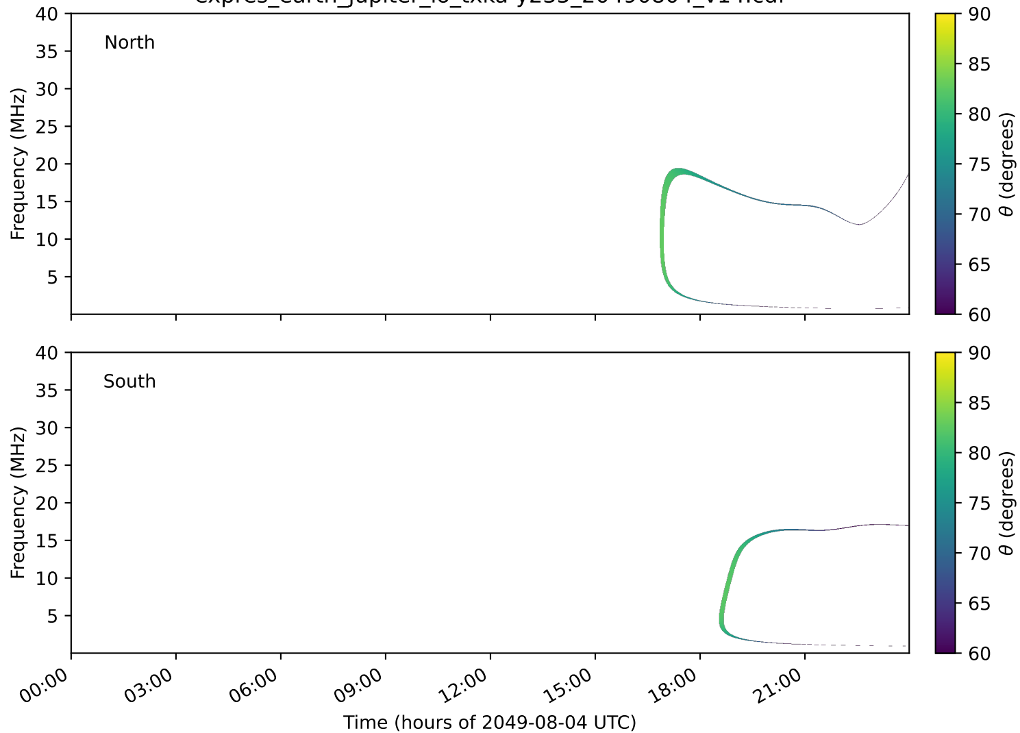
expres_earth_jupiter_io_txka-y235_20490804_v14.cdf
