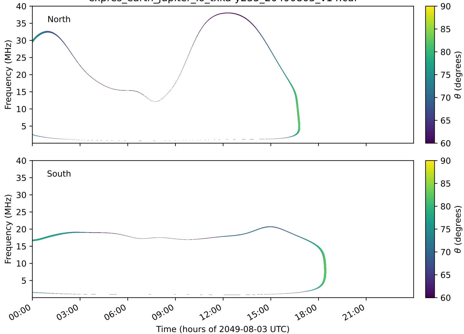
expres_earth_jupiter_io_txka-y235_20490803_v14.cdf
