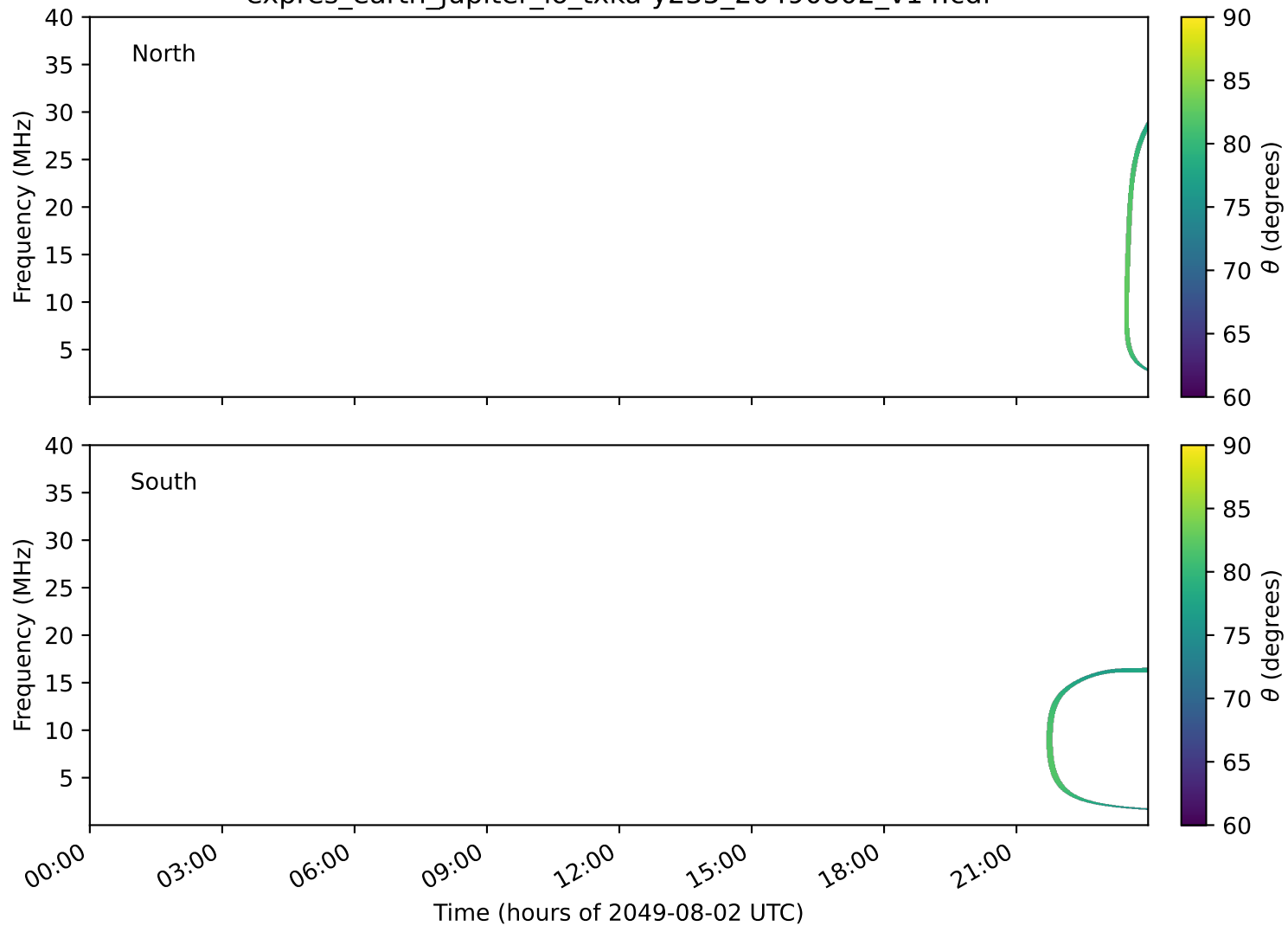
expres_earth_jupiter_io_txka-y235_20490802_v14.cdf
