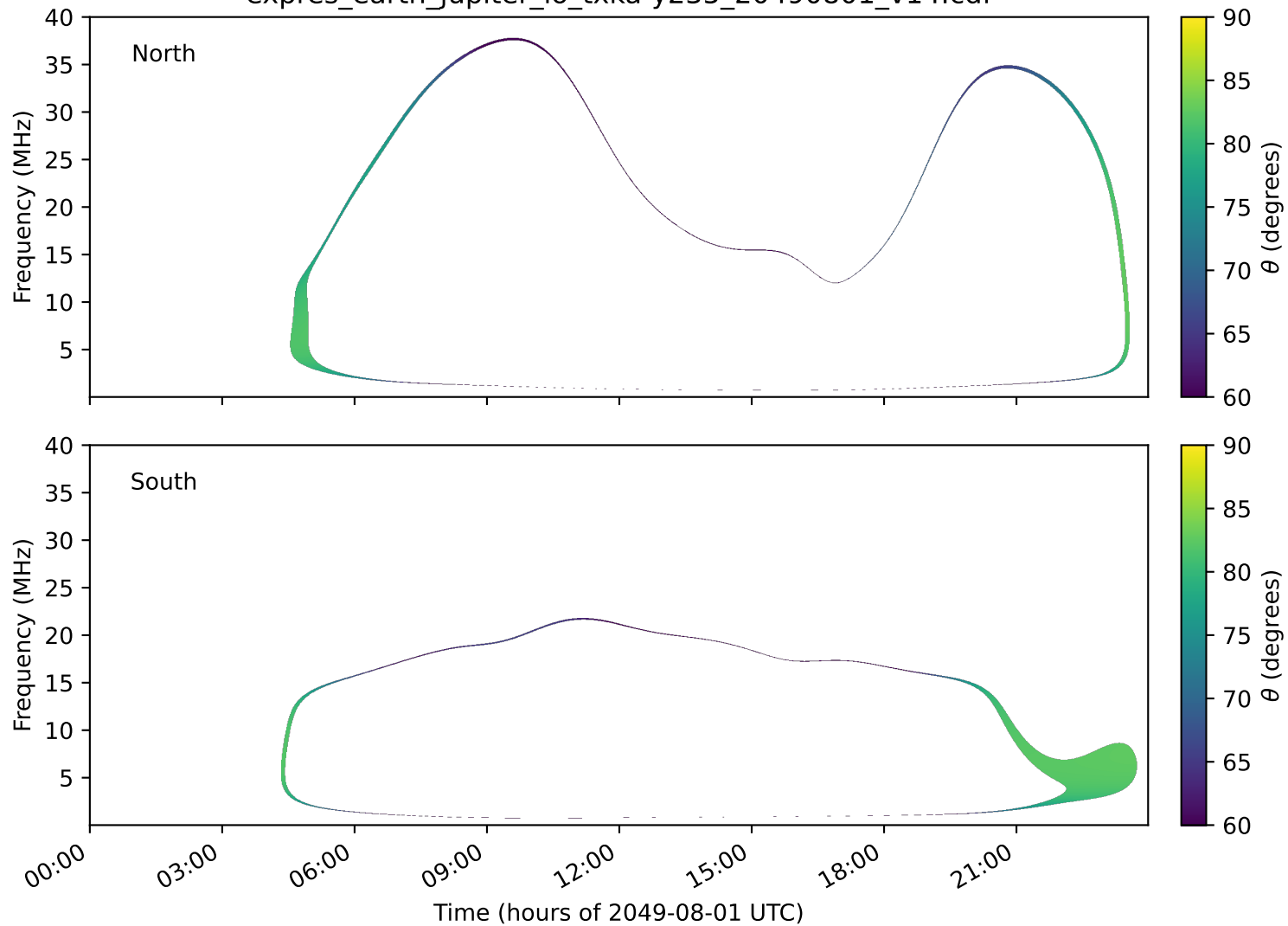
expres_earth_jupiter_io_txka-y235_20490801_v14.cdf
